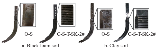
Figure 5 Surface morphology of O-S and C-S-T-SK-2# after subsoiling in black loam soil and clay soil
