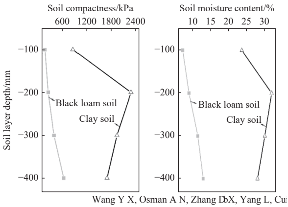
Figure 2 Soil compactness and moisture content in different tillage layers of black loam and clay soil
