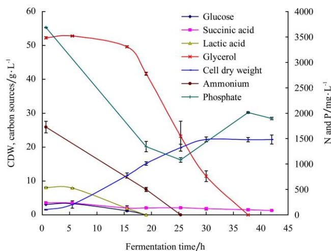
Figure 2 Growth of P. putida KT217 on a 400g/L CCS based medium (108.4 g/L dry wt) with 1.73 g/L of ammonia added. Points are the means of measurements obtained from three separate trials. Nitrogen and phosphorus are shown on the right-hand axis
